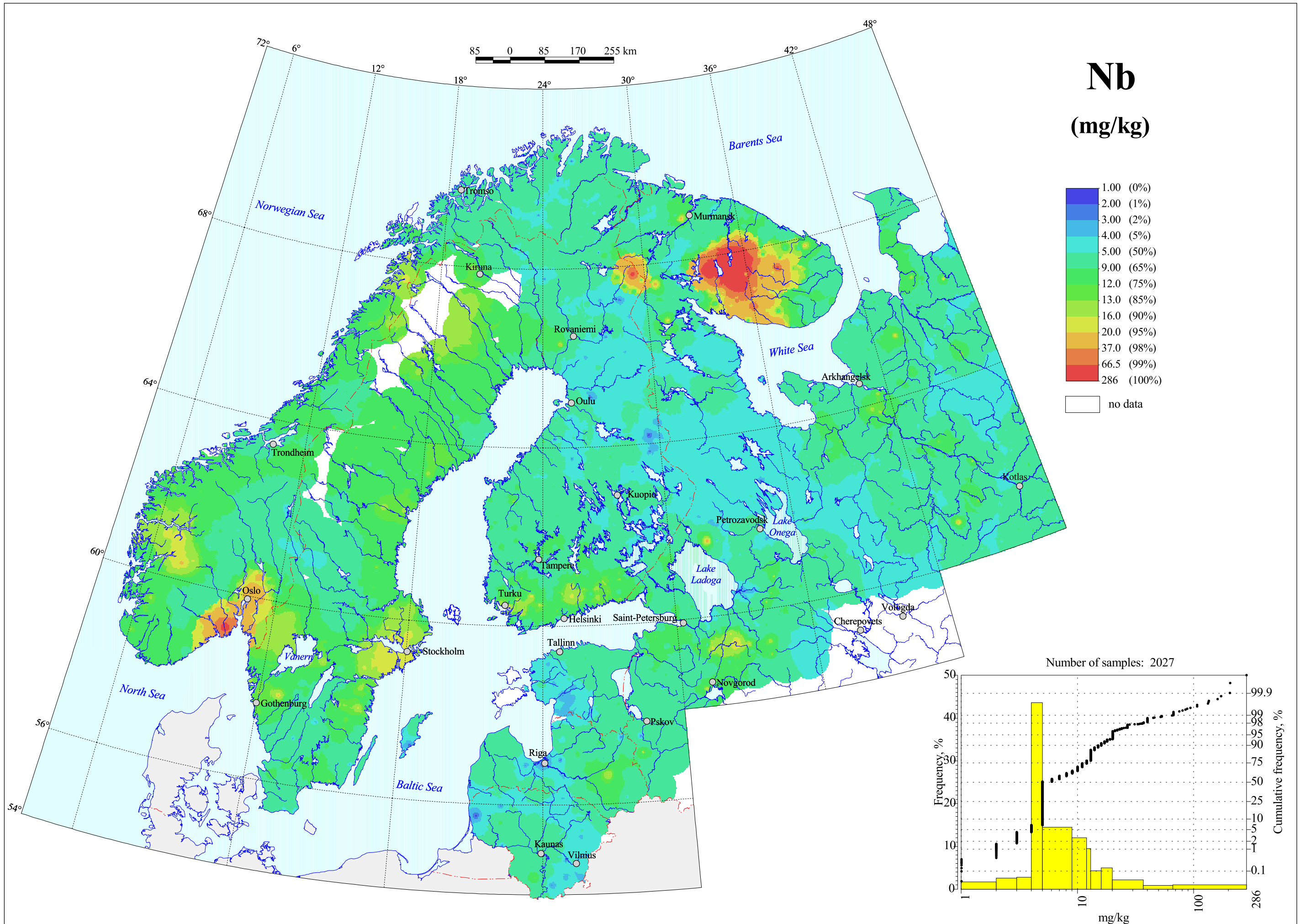
Niobium in C-horizon, Grain Size <2 mm, Total Content
